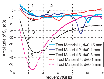
Figure 12. Comparison of the modeled attenuation on the line with different test materials.
