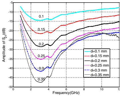
Figure 13. Predicted attenuation on the line with Test Material 3 of different thickness d .
