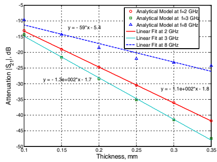
Figure 14. Predicted attenuation as the function of the thickness d of Test Material 3 for a few frequency points.
