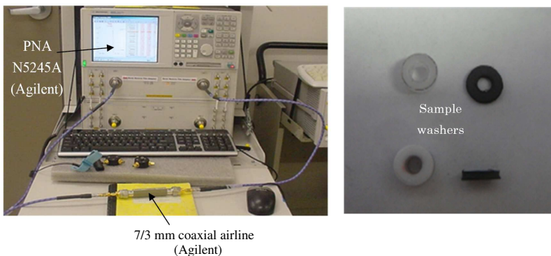
Figure 3. Experimental setup and samples (washers) for measuring dielectric and magnetic properties of absorbing materials.
