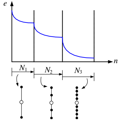
Figure 5. Optimization design process according to extension of the lattice.
