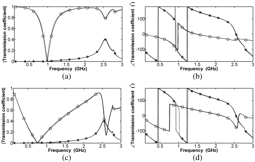
Figure 2. Co-polarized and cross-polarized transmission coefficient results for the LE-PL-OWG FSS with Z_{v(A)} = Z_{v(B)} = 1/(j\omega C) , C = 1 pF, l = 1.25 mm, b = 0.36 mm, D_x = D_z = 60 mm, \xi = 70^\circ , \psi = 22.5^\circ , y_{obs} = 20 mm. The surrounding medium is free space. CST: Dashed line. WH method: Solid line. Q = 10 , Q' = 20 \times Q , Q_\Delta = 20 \times Q . (a) Magnitude of T_{\parallel\parallel} : (o) and T_{\perp\parallel} : (*). (b) Phase of T_{\parallel\parallel} : (o) and T_{\perp\parallel} : (*). (c) Magnitude of T_{\perp\perp} : (o) and T_{\parallel\perp} : (*). (d) Phase of T_{\perp\perp} : (o) and T_{\parallel\perp} : (*).
