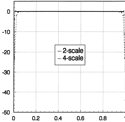
Figure 10a. The solution of the coefficients in different scales.
