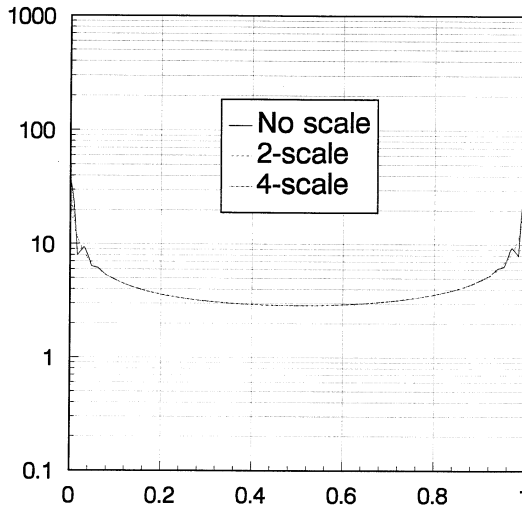
Figure 7b. The solution of the equation on different scales, initial number of nodes, N = 64 .
