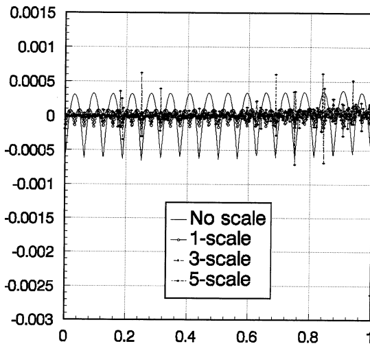
Figure 4b. The difference between the exact solution and the solutions of equation in different scales. Initial number of nodes, N = 16 .
