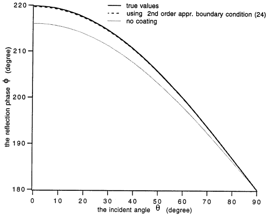
Figure 2. The reflection phase \phi as a function of the incident angle \theta . The dashed curve is obtained by using the effective boundary condition (24). The solid curve is for the true values calculated with a shooting method.
