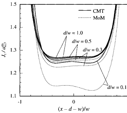
(c) J_z for the asymmetric mode.
