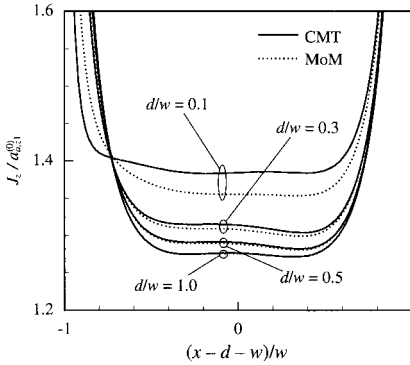
(a) J_z for the symmetric mode.
