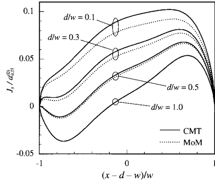
(b) J_x for the symmetric mode.
