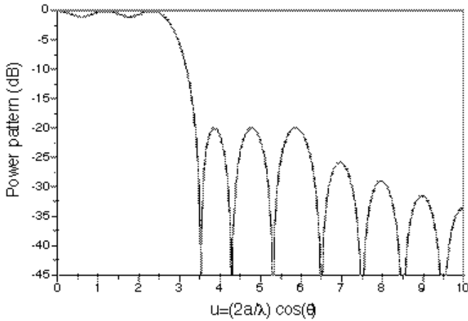
Figure 3. Flat-topped beam obtained in Section 3.2. Ripple, \pm 0.5 dB; side lobe level, -20 dB.
