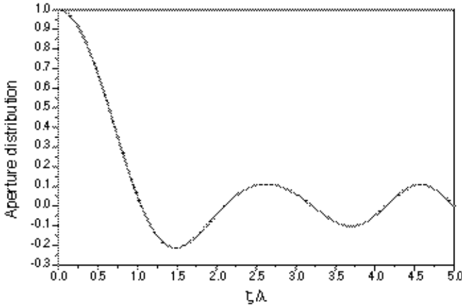
Figure 7. Amplitude of the aperture distribution affording the radiation pattern of Fig. 6.
