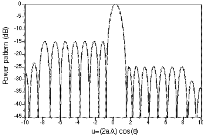
Figure 8. Asymmetric sum pattern obtained in Section 3.4. Side lobe levels, -15 and -25 dB.
