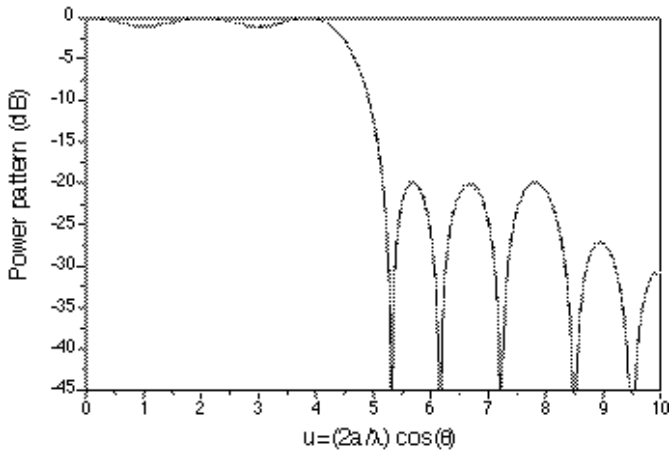
Figure 6. Flat-topped beam obtained in Section 3.3 using a real aperture distribution. Ripple, \pm 0.5 dB; side lobe level, -20 dB.
