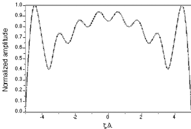
Figure 9. Amplitude of the aperture distribution affording the radiation pattern of Fig. 8.
