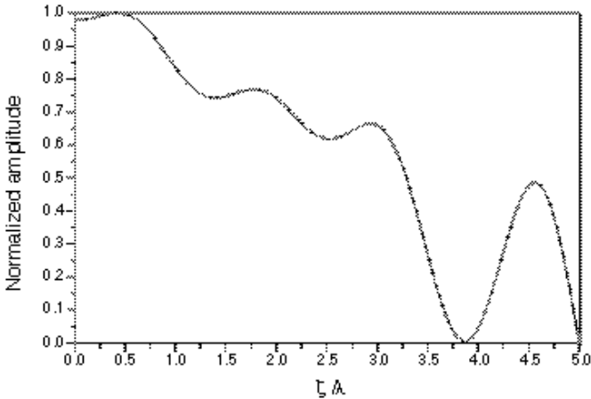
Figure 2. Amplitude of the aperture distribution affording the radiation pattern of Fig. 1.
