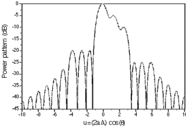
Figure 11. Cosec-squared pattern obtained in Section 3.5. Ripple, \pm 1 dB; side lobe levels, -20 and -25 dB.
