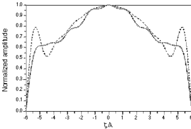
Figure 18. Amplitudes of the aperture distributions affording the radiation patterns of Fig. 17. Note the reduction in edge-brightening.
