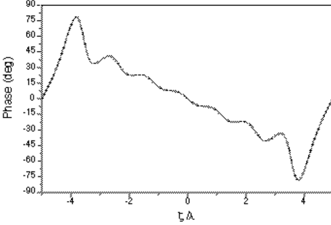
Figure 10. Phase of the aperture distribution affording the radiation pattern of Fig. 8.
