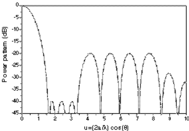
Figure 1. Symmetric sum pattern obtained in Section 3.1.
