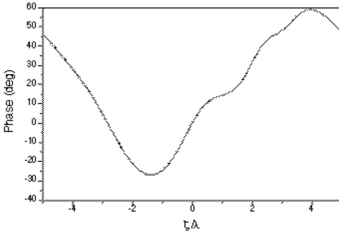
Figure 13. Phase of the aperture distribution affording the radiation pattern of Fig. 11.
