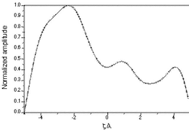
Figure 12. Amplitude of the aperture distribution affording the radiation pattern of Fig. 11.
