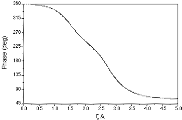
Figure 5. Phase of the aperture distribution affording the radiation pattern of Fig. 3.
