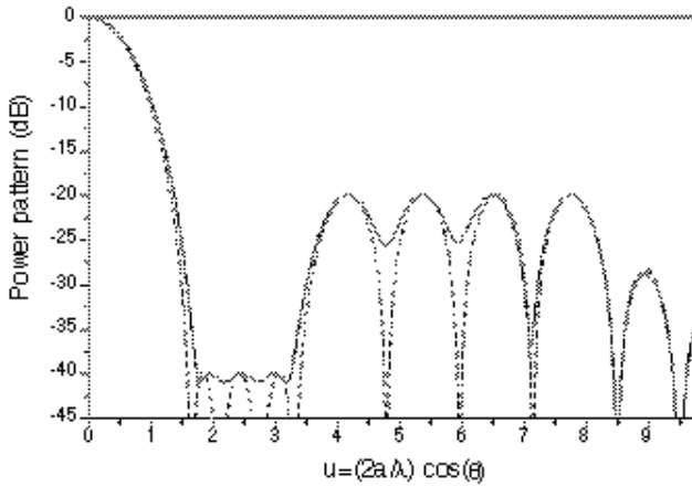
Figure 14. Symmetric sum pattern obtained in Section 3.6 while minimizing the variation (—), and the pattern obtained in Section 3.1 without aperture optimization (- - -).
