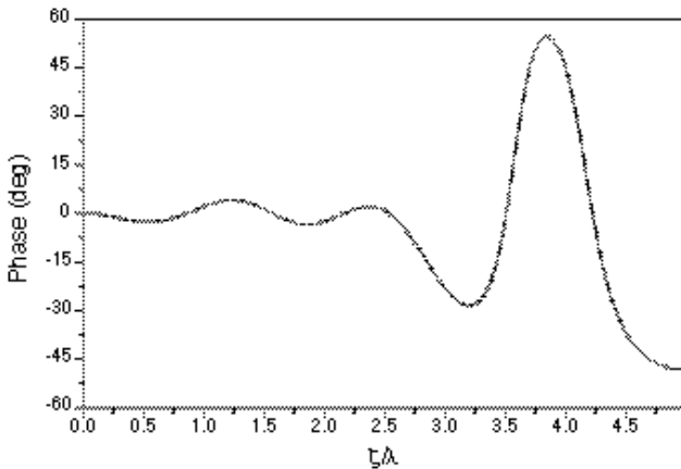
Figure 16. Phase of the aperture distribution affording the radiation pattern of Fig. 14.
