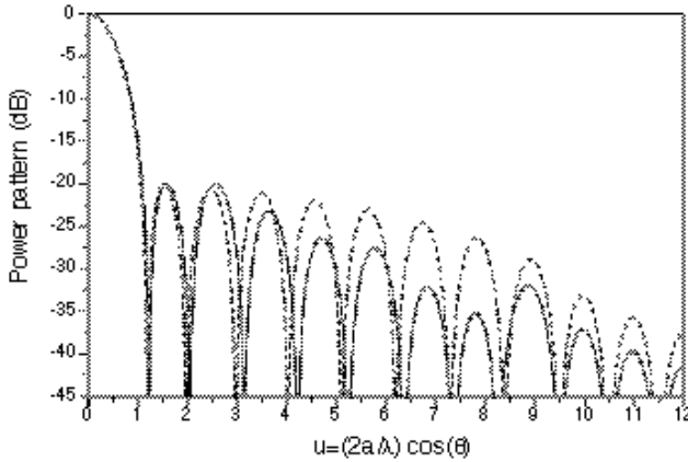
Figure 17. Symmetric sum pattern similar to a Rhodes pattern obtained with a smooth aperture distribution in Section 3.7 (—), and the original -20 dB \bar{n} = 9 Rhodes pattern used as starting point.
