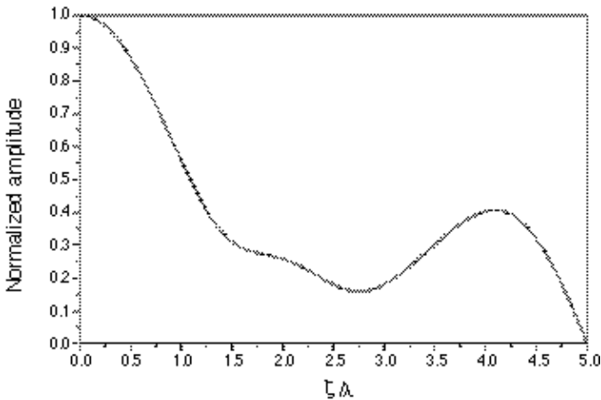
Figure 4. Amplitude of the aperture distribution affording the radiation pattern of Fig. 3.
