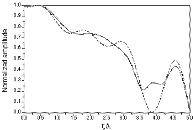
Figure 15. Amplitudes of the aperture distributions affording the radiation patterns of Fig. 14. Note the reduction in edge-brightening.
