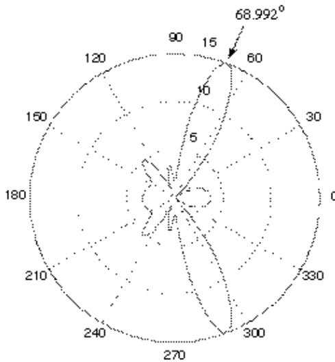
Figure 8. Radiation pattern for the azimuth plane of a linear array of 10 dipoles with direction of maximum gain at 68.992^\circ ( V = 1001111010 ).
