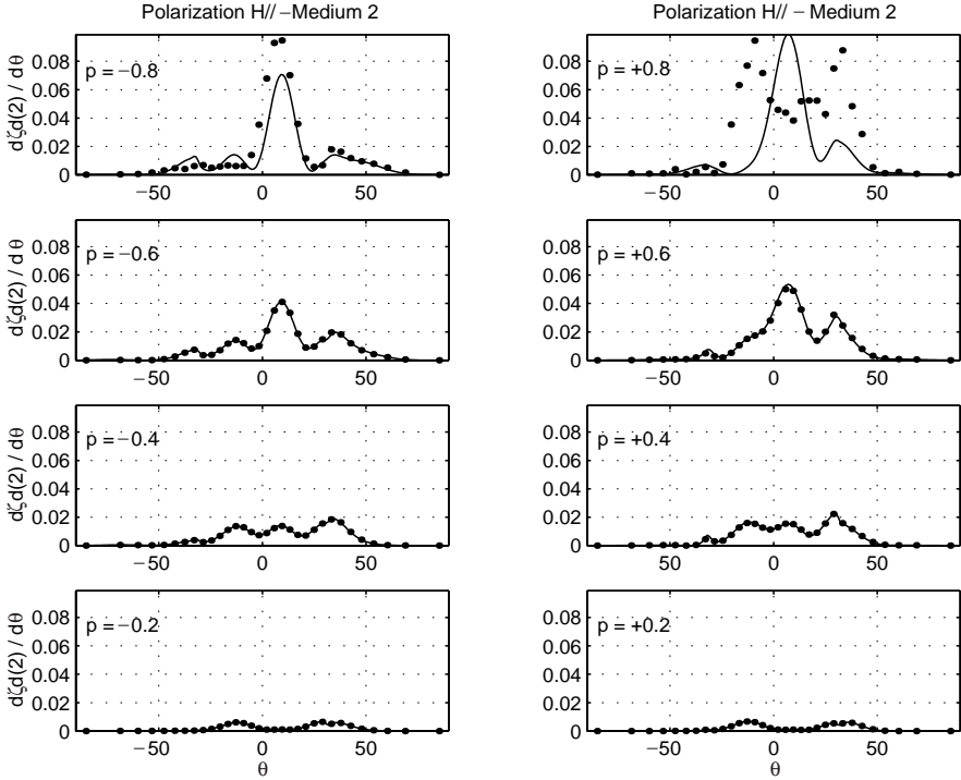
Figure 7. Normalized scattering patterns \frac{d\xi_d^{(2)}}{d\theta} for four values of \pm p of H_{\parallel} polarized profiles referred to in Subsection 5.3. Same values as in Fig. 5.
