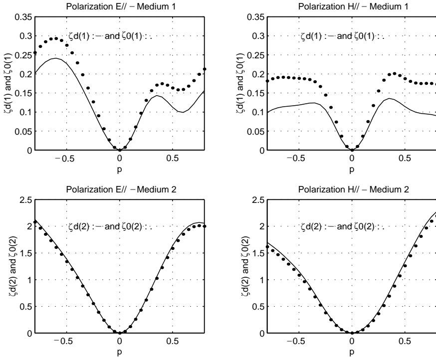
Figure 5. Total normalized power scattered in medium ( m ) \xi_d^{(m)} and normalized coupling power \xi_0^{(m)} as a function of the depth parameter p for the profile referred to in Subsection 5.3. M_c = 16 , M = \text{Ent}(|p|/\lambda + 2)M_c ; l = D = 20 cm, \lambda = 10 cm, \theta_i^{(1)} = 17.6^\circ , n_2 = 1.94 .
