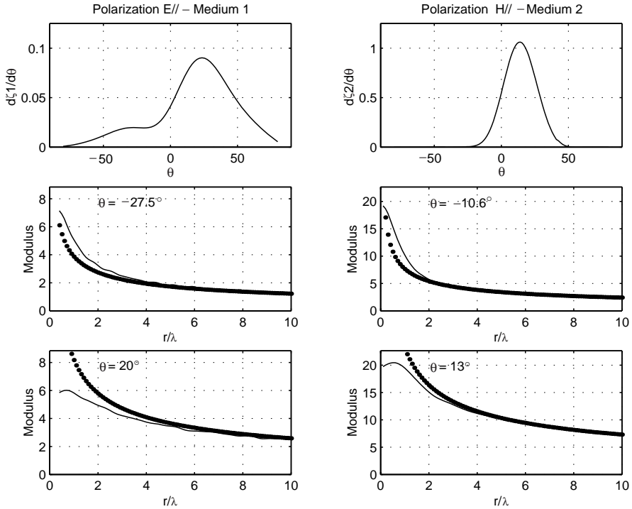
Figure 10. Normalized scattering patterns and magnitudes of F_d^{(m)}(r, \theta) and F_{d_{far}}^{(m)}(r, \theta) in both media as a function of r under many observation angles. Same values as in Fig. 8.
