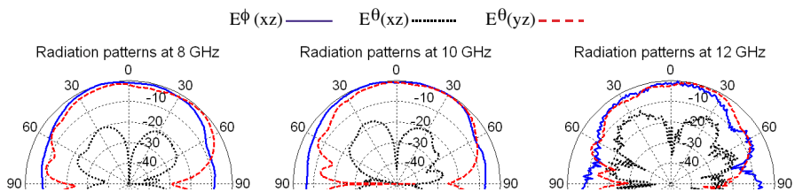
Figure 9. Measured radiation patterns in the X-band.
