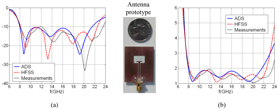
Figure 7. Comparison between the measured and computed (a) return loss, and (b) VSWR, for the rectangular slot antenna of W_1 , L_1 , W_2 , L_2 and L_3 = 11, 7, 6, 1, \text{ and } 1 .
