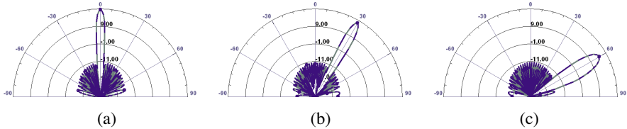
Figure 13. Computed copolarized gain in the x - z plane for 32-element array in x -direction at 10 GHz, with a steering angle of (a) 0^\circ , (b) 30^\circ , and (c) 60^\circ .
