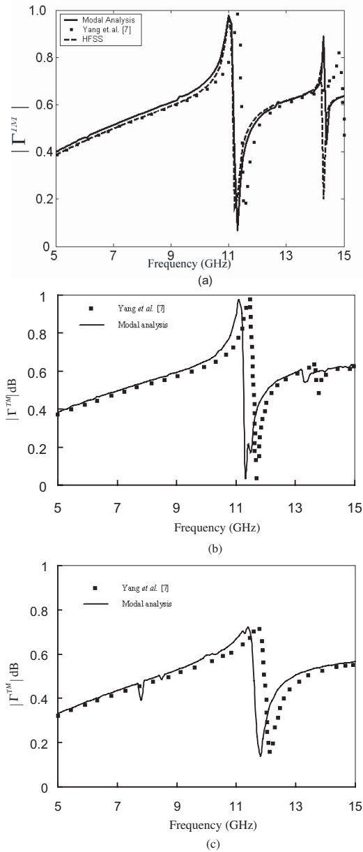
Figure 4. TM reflection coefficients of a two-dimensional grating with \epsilon_{rb} = 4 , \epsilon_{r1} = 10 , D_x = D_y = 20 mm, l_{x1} = 10 mm, l_{y1} = 10 mm, x_{01} = 10 mm, y_{01} = 10 mm and h = 2 mm. \phi_{inc} = 0^\circ and (a) \theta_{inc} = 0^\circ , (b) \theta_{inc} = 15^\circ and (c) \theta_{inc} = 30^\circ .
