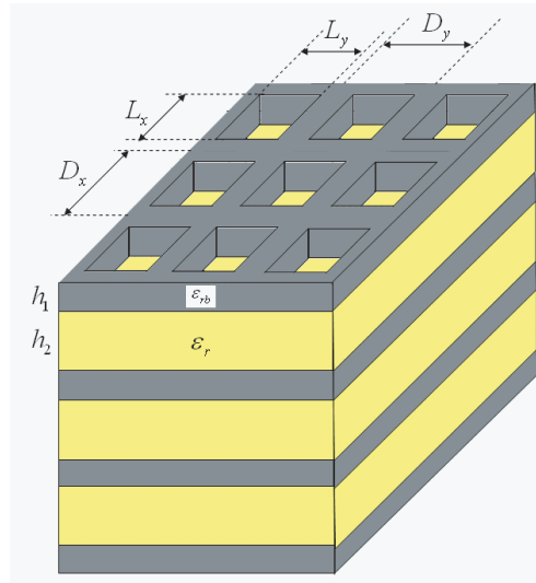
Figure 8. FSS of multilayered dielectric grating slabs. D_x = D_y = 10 mm, L_x = L_y = 7 mm, \epsilon_{rb} = 12 , h_1 = 2 mm, \epsilon_r = 2.2 and h_2 = 4 mm.
