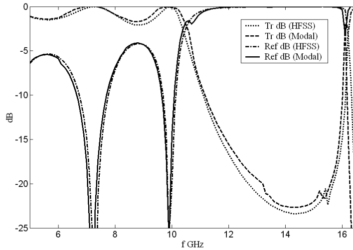
Figure 9. Reflection and Transmission coefficients of multilayered dielectric grating slabs shown in Fig. 8 for the case of normal incidence. \theta_{inc} = 0 and \phi_{inc} = 0 . The incident field is y -polarized field.
