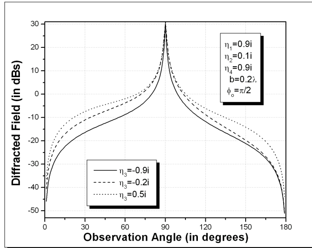
Figure 5b. The variation of the diffracted field with respect to \eta_3 .
