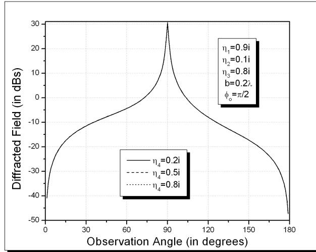
Figure 6. The variation of the diffracted field with respect to \eta_4 .
