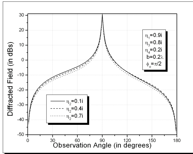
Figure 4a. The variation of the diffracted field with respect to \eta_2 .
