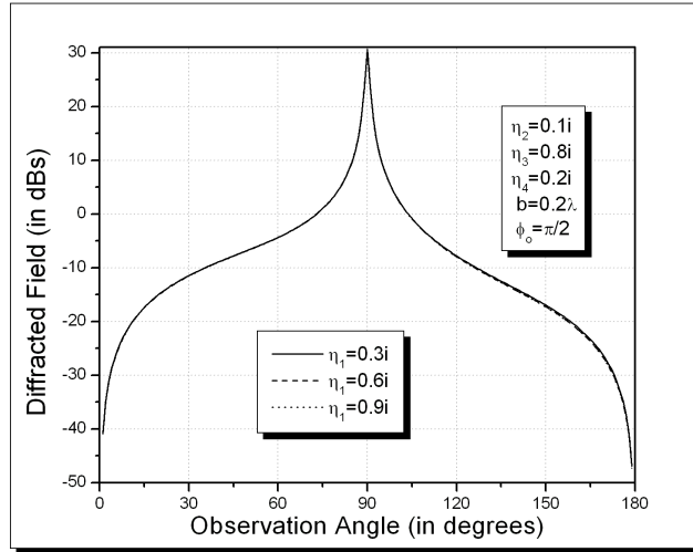
Figure 3. The variation of the diffracted field with respect to \eta_1 .
