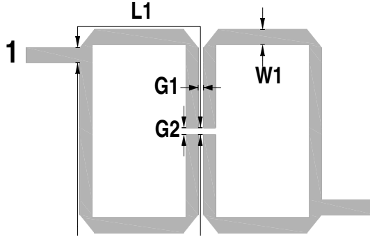
Figure 4. Layout of open-loop resonator bandpass filter.
