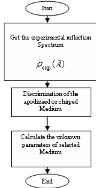
Figure 2. The scheme of inverse scattering with GA.
