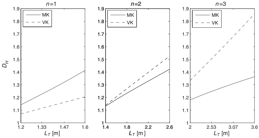
Figure 7. Hausdorff dimension of the two considered prefractal dipoles as a function of the total length for different values of n : MK — Minkowski, VK — Von Koch.
