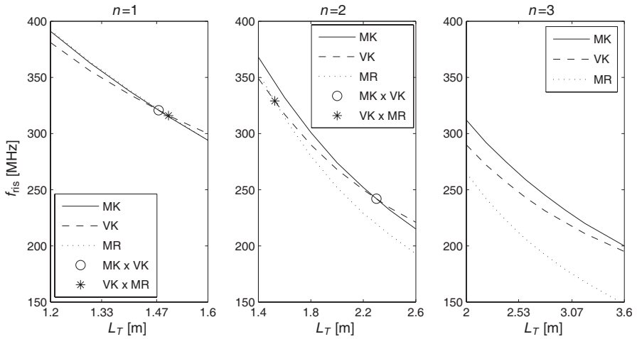
Figure 5. Second resonant frequency of the three considered dipoles as a function of the total length for different values of n : MK — Minkowski, VK — Von Koch, MR — meander line.
