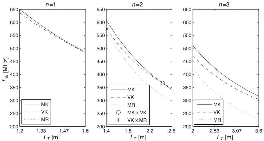
Figure 6. Third resonant frequency of the three considered dipoles as a function of the total length for different values of n : MK — Minkowski, VK — Von Koch, MR — meander line.
