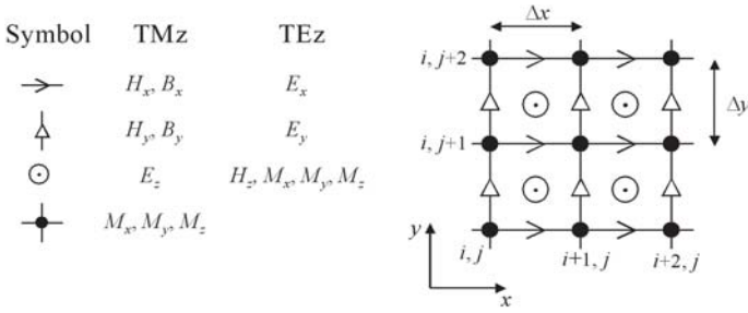
Figure 2. Two-dimensional FDTD grid showing TMz and TEz field symbols, including the proposed placement of the magnetisation vector at the cross points of the grid cells.
