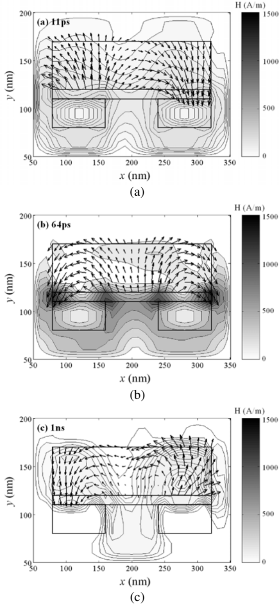
Figure 5. Magnetisation (arrow plot) and magnetic field magnitude (contour plot) distributions at three time instances: (a) 0.01 ns, (b) 0.064 ns and (c) 1 ns. Two point interpolations were carried out on the magnetic field components to evaluate them at the same location of the magnetisation. The PML region is not shown in these plots.
