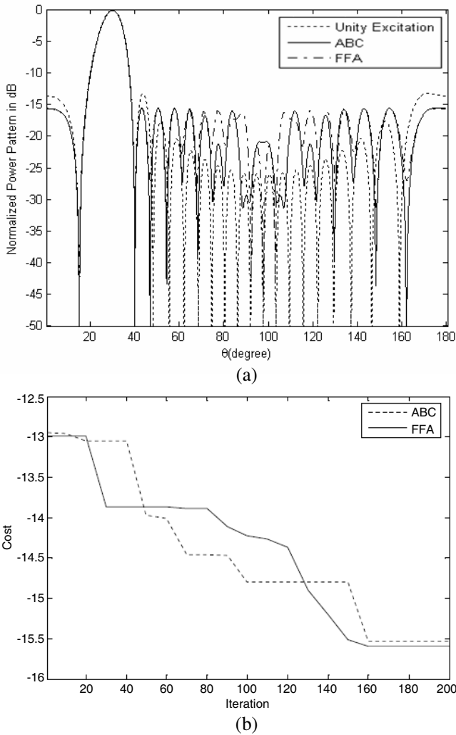
Figure 5. (a) Normalized Power Patterns steered at 30^\circ with 20 elements array using FFA and ABC. (b) Convergence curves of the scanned array steered at 30^\circ with 20 elements using FFA and ABC.
