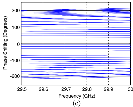
Figure 9. The phase shifting of three types of phase shifters versus frequency, (a) Chebyshev with the order of 5, the return loss of 10 dB, the bandwidth of 2 GHz, and Q_u equal to 200, (b) Elliptical with the order of 6, the return loss of 10 dB, the bandwidth of 2 GHz, and Q_u equal to 200, and (c) 2nd order All-Pass circuit ( \sigma_b = 24 , \omega_b = 26 ).
