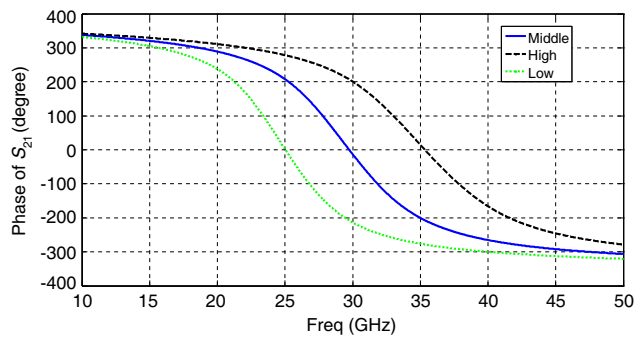
Figure 7. Phase response of the typical 2nd order All-Pass circuit.
