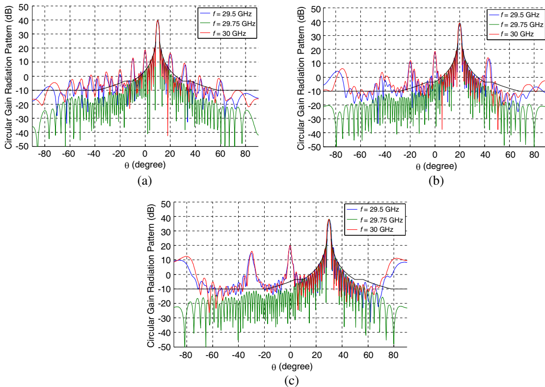
Figure 10. Gain radiation pattern at f = 29.5, 29.75, \text{ and } 30 GHz for Chebyshev phase shifter when the scanning angle is (a) 10^\circ , (b) 20^\circ , (c) 30^\circ .
