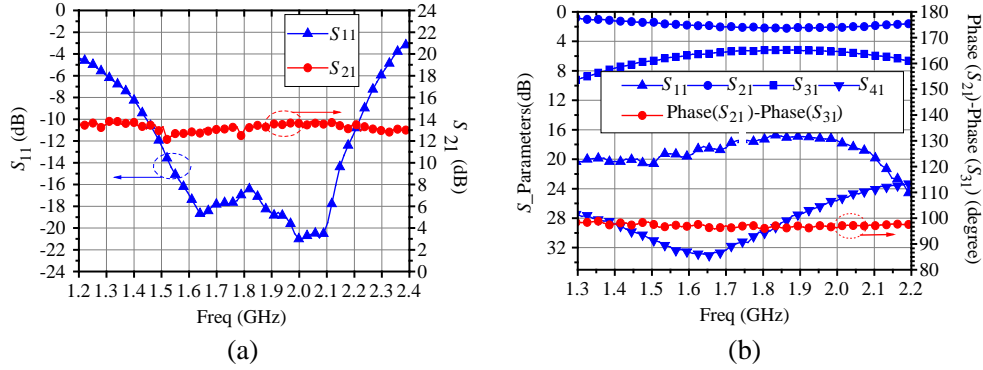
Figure 3. Measured small-signal S -parameters of (a) single power amplifier (CPA or PPA) biased at class-AB condition, (b) microstrip coupled-line coupler.
