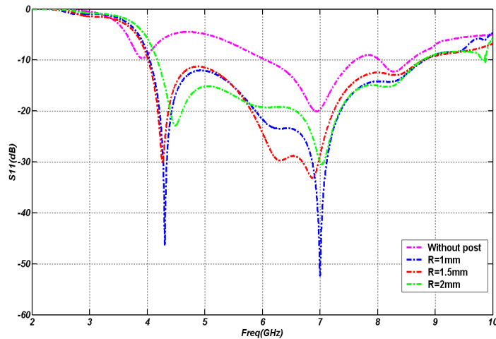
Figure 5. Return Loss of the antenna for various diameters of the posts. W1 = 22 mm, W2 = 11.5 mm, P = 5 mm, H = 8 mm, X = 5.7 mm, X1 = 4.5 mm, X2 = 2 mm, Y1 = 4 mm, Y2 = 8 mm.
