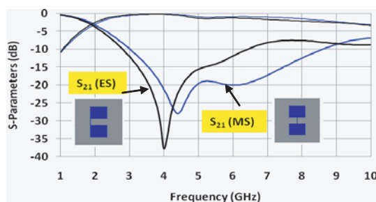
Figure 1. The simulated S -parameters for slot under line is in the middle (MS) or at the edge (ES) of two 8 \times 8 \text{ mm} square dumbbell slots.
