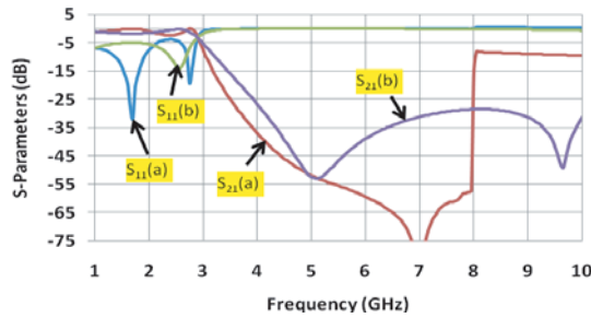
Figure 9. The simulated S -parameters for the equivalent circuits of Fig. 8.
