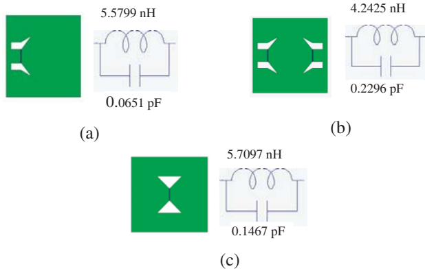
Figure 7. The equivalent circuit for dumbbell slots, (a) one reshaped dumbbell slot, (b) two reshaped dumbbell slots, (c) triangle dumbbell slot.
