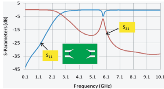
Figure 5. The simulated S -parameters for the reshaped rectangular dumbbell slots.
