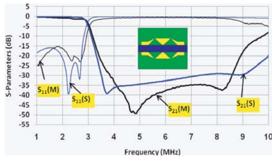
Figure 10. The measured and simulated S -parameter for the defected ground lowpass filter.
