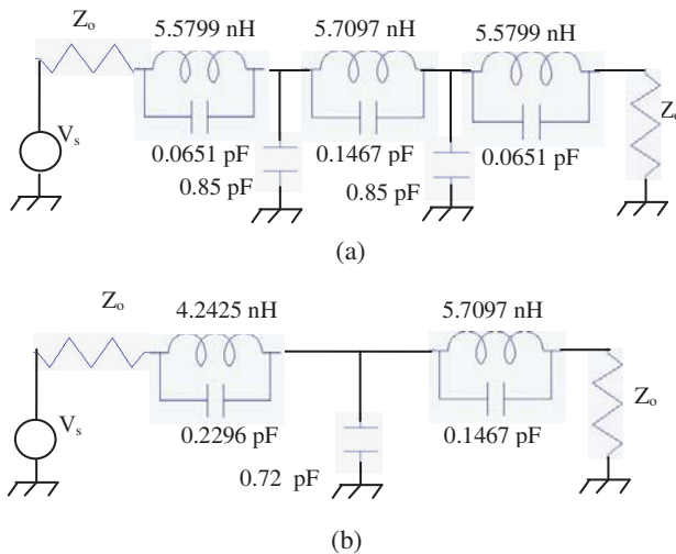
Figure 8. The equivalent circuit for the lowpass filter with three dumbbell slots.
