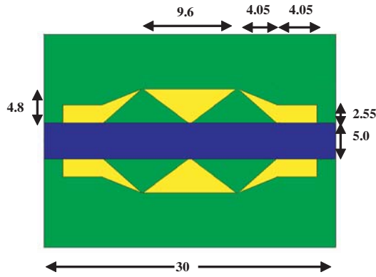
Figure 3. The geometric dimension of the reshaped dumbbell slots, all dimension are in (mm).
