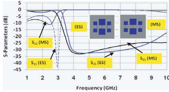
Figure 2. The simulated S -parameters for each of (MS) or (ES) when use three periodic dumbbell slots.
