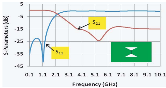
Figure 4. The simulated S -parameters for the inverted triangle dumbbell slots.
