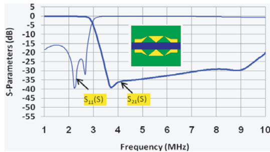
Figure 6. The simulated S -parameters for the the three dumbbell slots.
