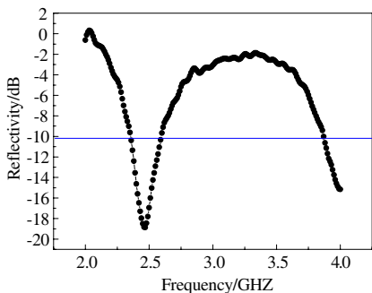
Figure 3. Reflectivity of the asphalt mixes at different frequency.
