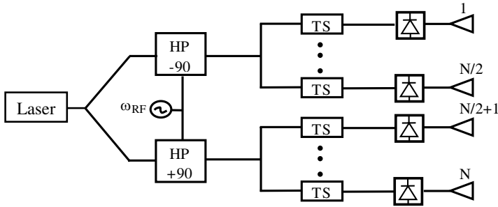
Figure 17. Scheme of the optical architecture proposed to realize both wide band sum and difference pattern: In the graph the HPs are set in order to get a difference pattern.
