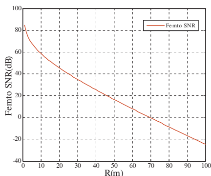
Figure 14. SNR vs. Distance in femto cell.
