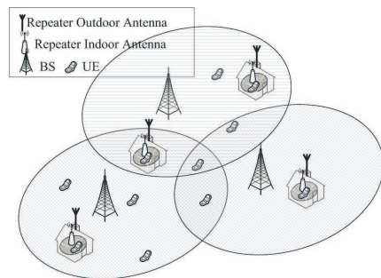
Figure 11. The repeaters installed environment.
