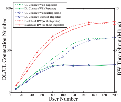
Figure 12. Users service quantity and throughput with and without installation of repeaters.
