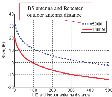
Figure 10. The output SNR of indoor antenna.
