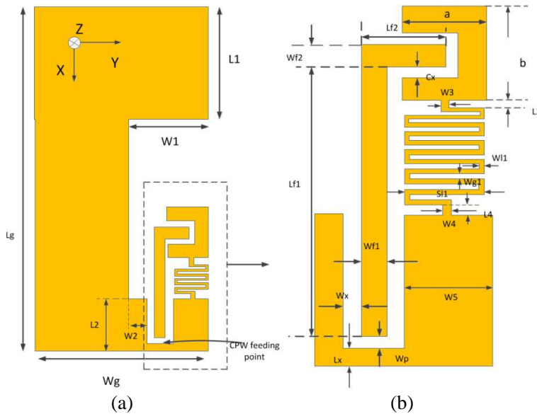
Figure 1. The configuration of the proposed antenna. (a) The overview. (b) The detail of parasitic element and L-shape monopole.
