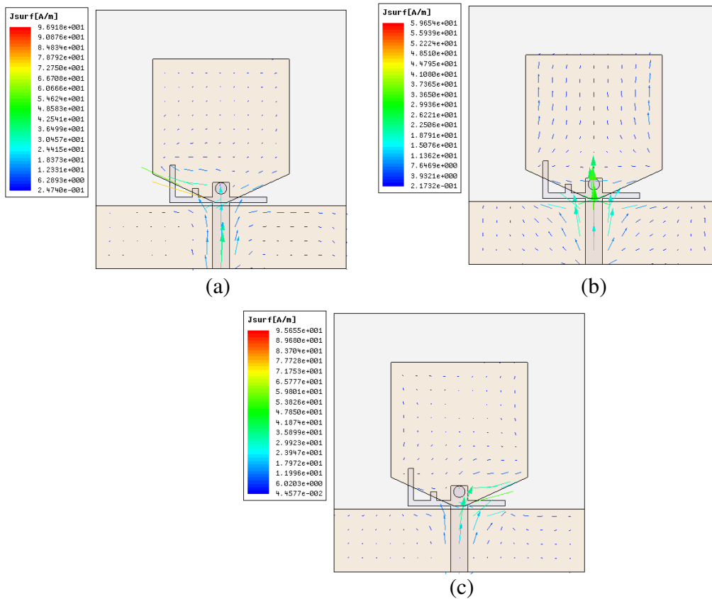
Figure 12. Simulated current distributions at (a) f = 2.8 GHz, (b) f = 4 GHz, (c) f = 5.5 GHz.
