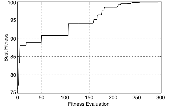
Figure 4. Convergence curve.
