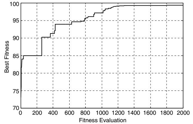
Figure 6. Convergence curve.
