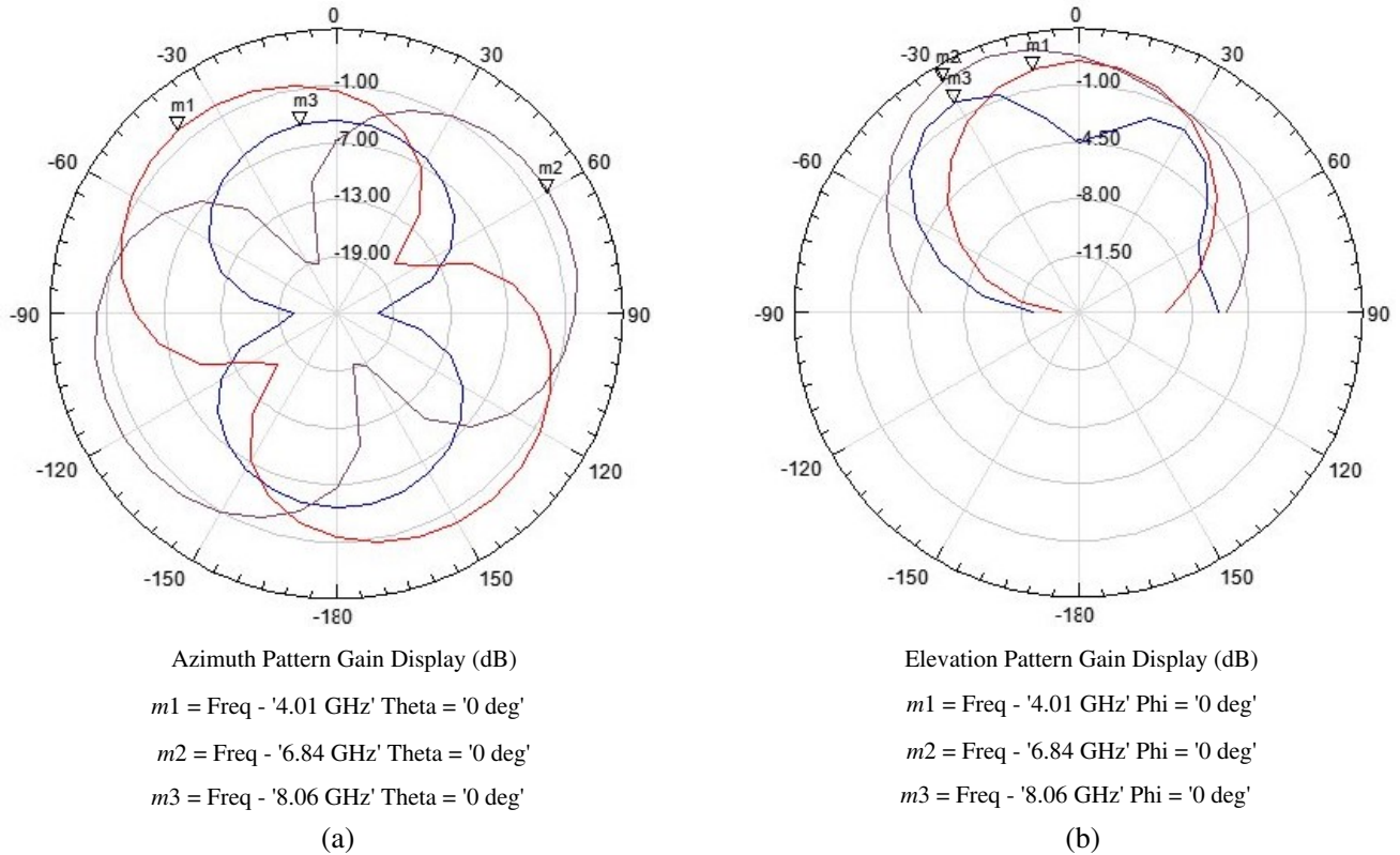
Figure 12. Radiation patterns of metamaterial loaded square shaped fractal antenna with 2nd iteration, (a) azimuth, (b) elevation.
