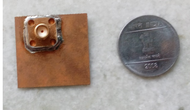
Figure 7. Bottom view of fabricated square shaped fractal antenna with 2nd iteration.
