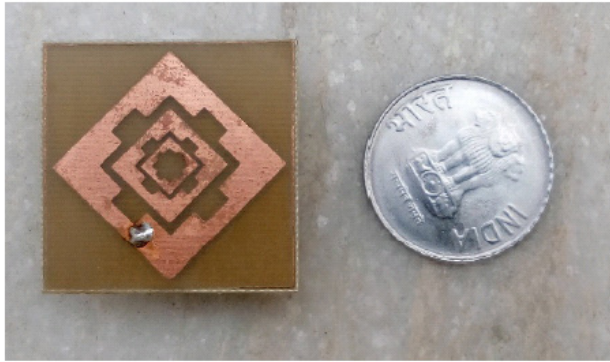
Figure 6. Photograph of fabricated square shaped fractal antenna with 2nd iteration.
