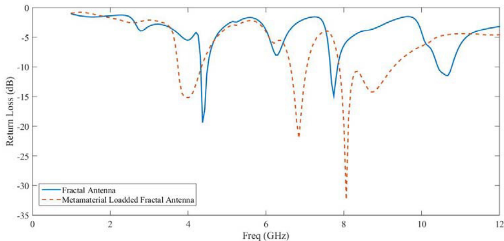
Figure 8. Comparison of simulated return loss of square shaped fractal antenna and metamaterial loaded square shaped fractal antenna with 2nd iteration.
