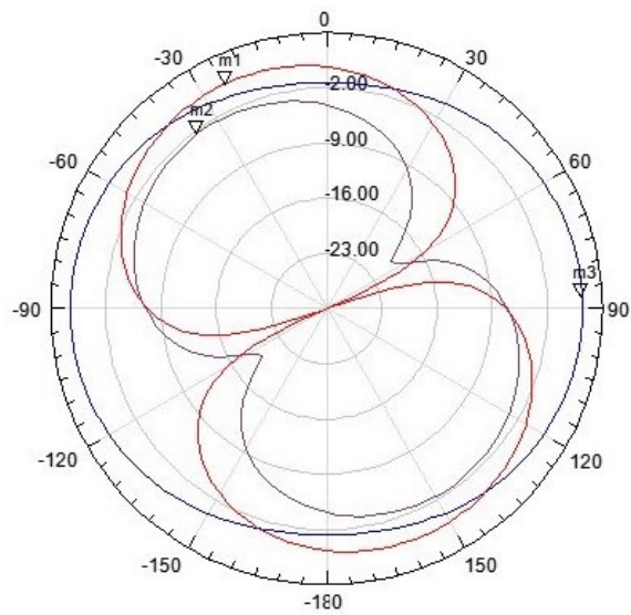
Azimuth Pattern Gain Display (dB) m1 = Freq - '4.371 GHz' Theta = '0 deg' m2 = Freq - '7.74 GHz' Theta = '0 deg' m3 = Freq - '10.67 GHz' Theta = '0 deg'
