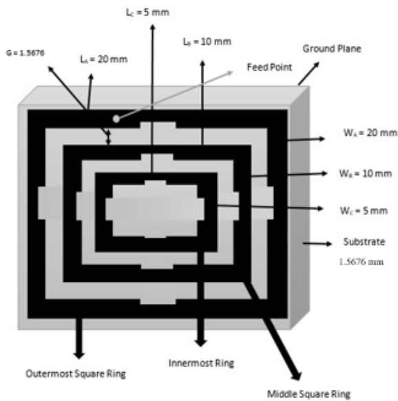
Figure 2. Square shaped fractal antenna with 2nd iteration.
