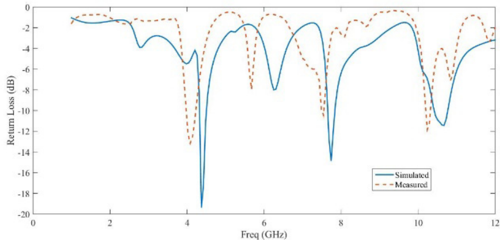
Figure 5. Comparison of simulated and measured return loss of square shaped fractal antenna with 2nd iteration.
