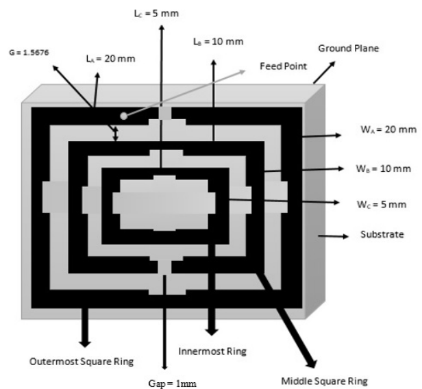
Figure 3. Metamaterial loaded square shaped fractal antenna with 2nd iteration.
