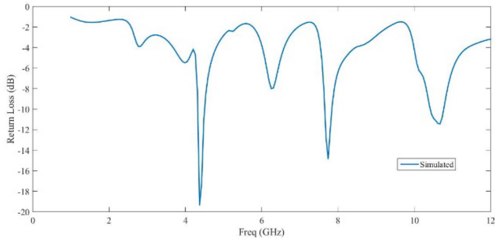
Figure 4. Return loss ( S_{11} ) of square shaped fractal antenna with 2nd iteration.
