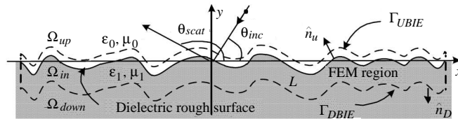
Figure 1. Geometry of scattering from a dielectric rough surface.
