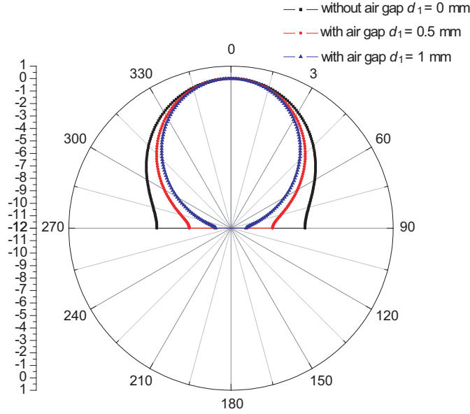
Figure 3. Radiation pattern ( E plane) versus air gap thickness; a = 50 mm, d_2 = 1.59 mm, \varepsilon_r = 2.32 .
