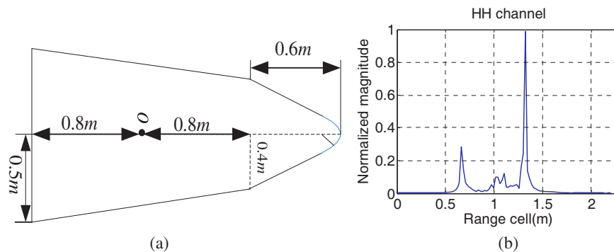
Figure 6. Target shape and range profile of static state. (a) The target model measured in microwave anechoic chamber, (b) range profile when the azimuth is 90° (HH channel).
