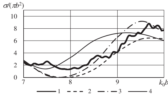
Figure 4. Normalized RCS of spherical screen versus k_0b (1 — measurement data [14]; 2 — results of computation given aluminum screen with the reflector’s edge of first kind; 3 — results of computation given aluminum screen with the reflectors edge of second kind; 4 — results of computation given perfectly conducting screen of zero thickness [6]).
