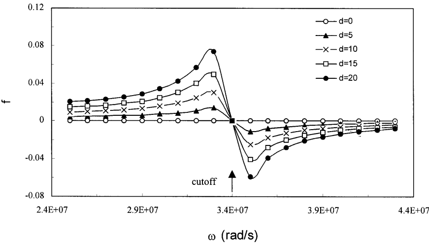
Figure 5b. The variations of f with frequency \omega and declination angle d .
