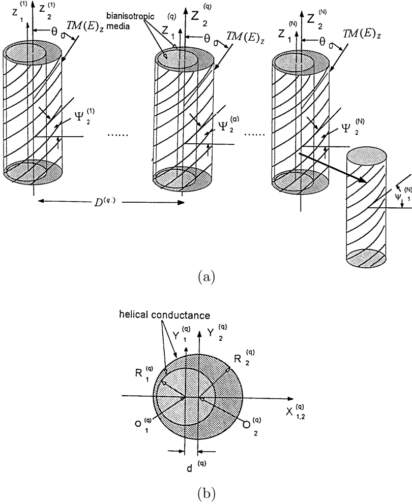
Figure 1. Geometry and co-ordinates of the linear array of N parallel eccentric bianisotropic cylinders with the helical conductances at \rho_1^{(q)} = R_1^{(q)} and \rho_2^{(q)} = R_2^{(q)} , respectively, The separation between the cylinders C^{(q)} and C^{(N)} is noted by D^{(Nq)} = |D^{(N)} - D^{(q)}| .
