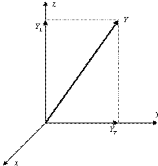
Figure 1. Geometry for the external magnetic field.
