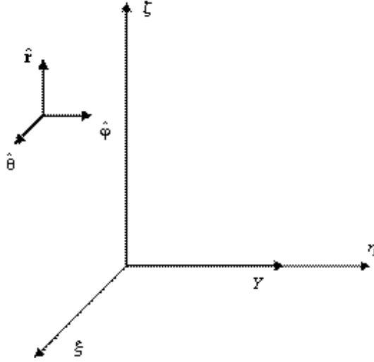
Figure 3. Geometry for spherical coordinates and circumferential external magnetic field.
