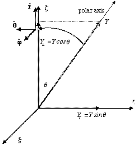
Figure 2. Geometry for spherical coordinates and external magnetic field along the \theta = 0 polar axis.
