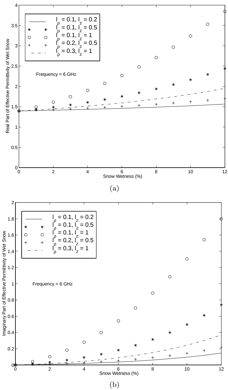
Figure 3. Effective permittivity of wet snow at 6 GHz with various correlation lengths (in mm). (a) Real part of the effective permittivity. (b) Imaginary part of the effective permittivity.
