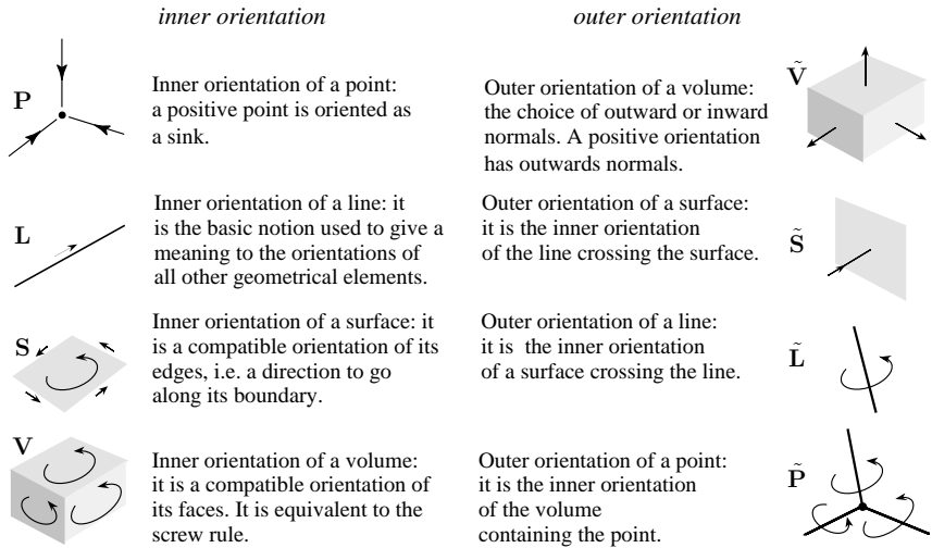
Figure 2. The two notions of inner and outer orientations in three-dimensional space.
