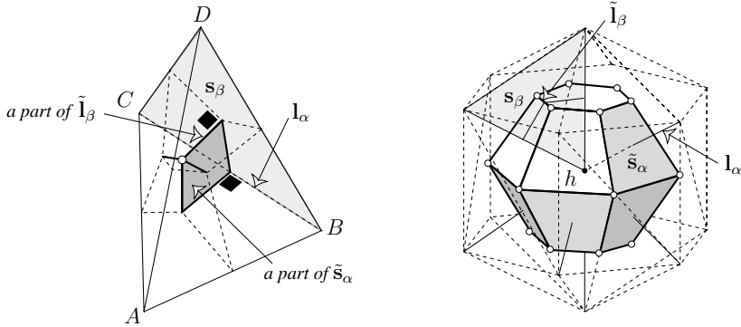
Figure 11. a) The six faces of a Voronoi cell contained in a tetraedron; b) the dual Voronoi cell \tilde{v}_h of a cluster of tetrahedra with a common vertex.
