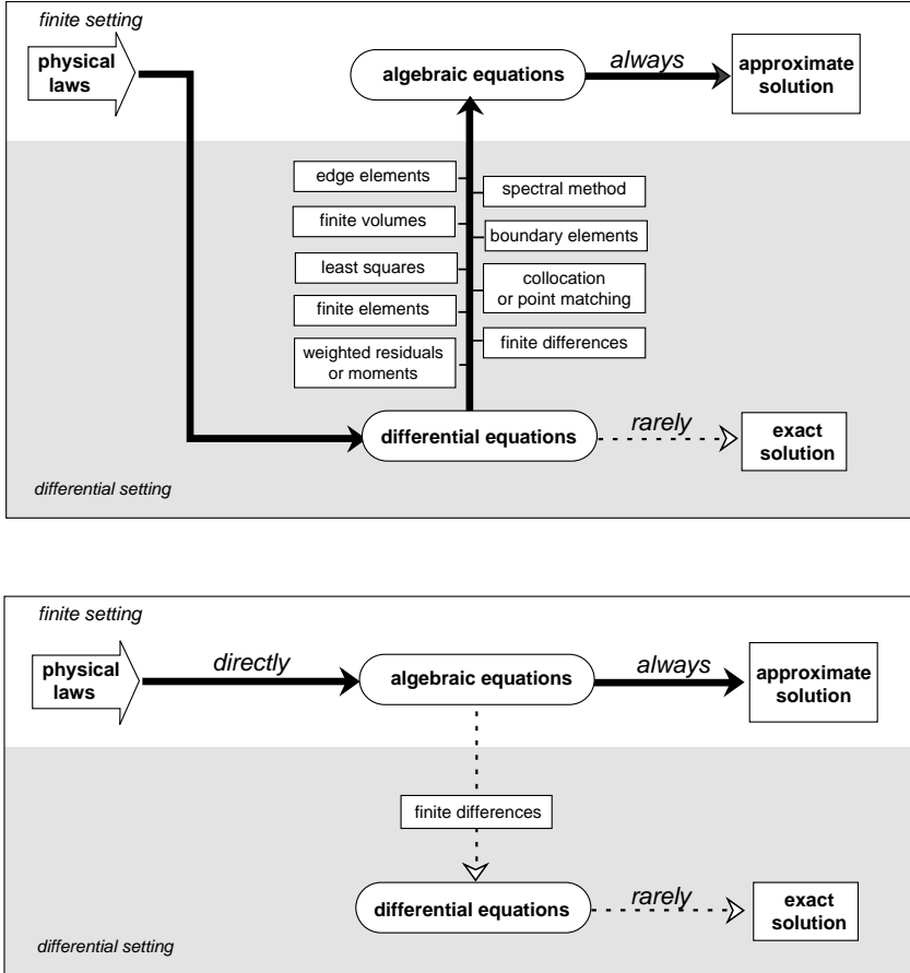
Figure 1. (above) In traditional differential formulation to obtain an approximate solution one is forced to pass through one of many methods of discretization. (below) On the contrary, using global variables and complexes, one obtain a finite formulation directly.
