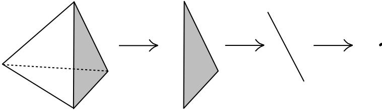
Figure 1. 3–, 2–, 1–, and 0– simplices
