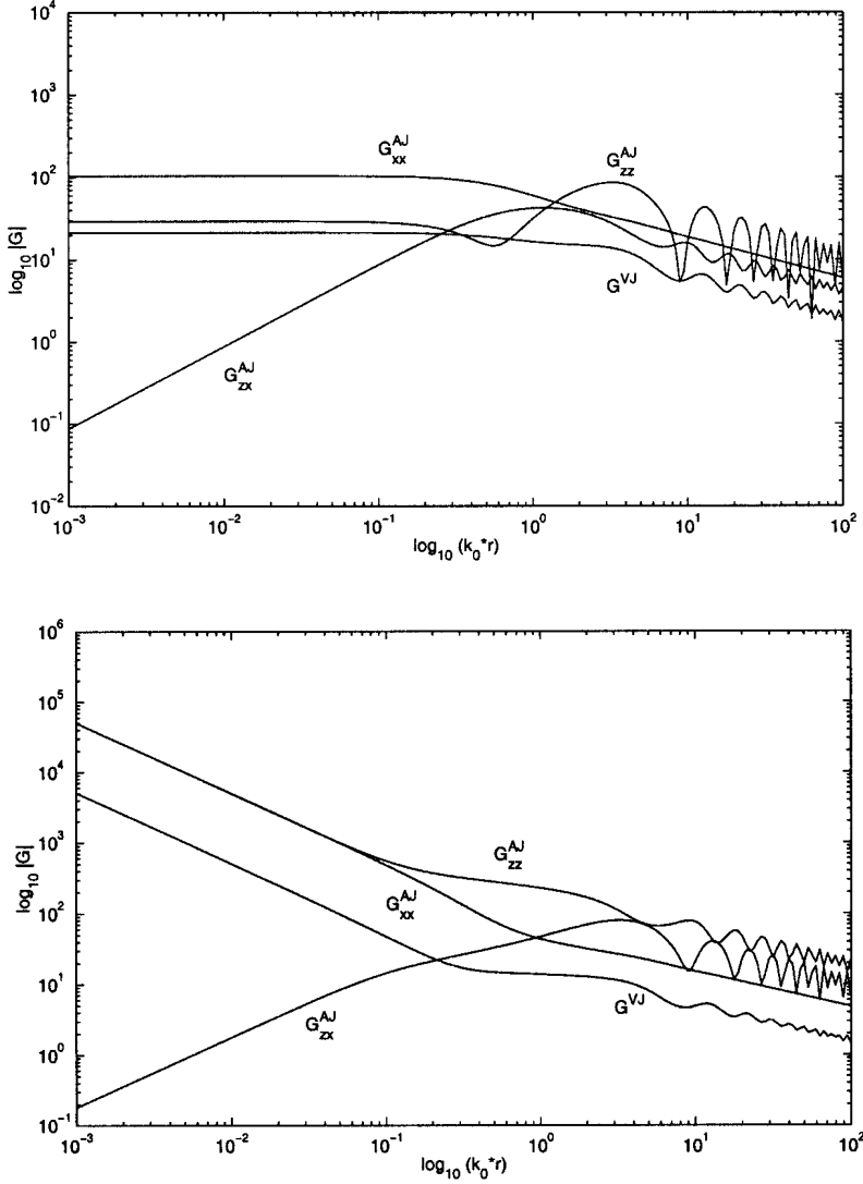
Figure 4. The magnitude of the Green's functions G^{VJ} , G^{AJ}_{xx} , G^{AJ}_{zz} and G^{AJ}_{zx} (multiplied by \varepsilon_0 ) in the 10 base logarithmic scale for the six layer structure of Figure 3. At the top z' = 0.4 mm, z = 1.4 mm (i.e., n = 3 , j = 5 ) and at the bottom z' = z = 0.4 mm (i.e., n = j = 3 ), respectively. Horizontal axis gives k_0 (wave number in vacuum) times r in the 10 base logarithmic scale and the frequency is 30 GHz.
