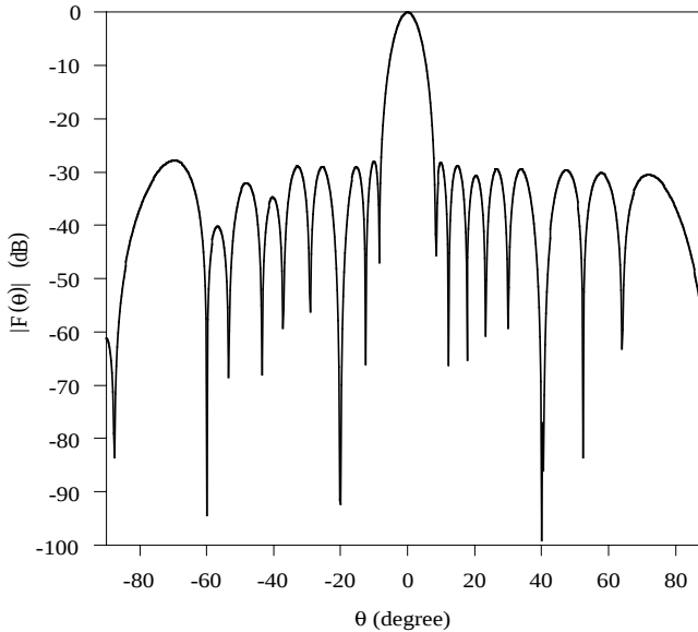
Figure 8. Radiation pattern obtained by controlling both the amplitude and phase with tripple imposed null at -60^\circ , -20^\circ and +40^\circ .
