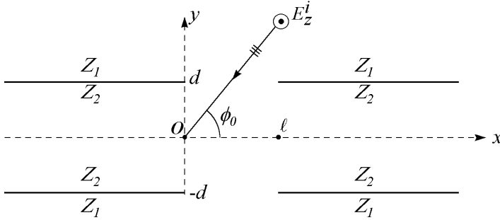
Figure 1. Tandem impedance slit waveguide.
