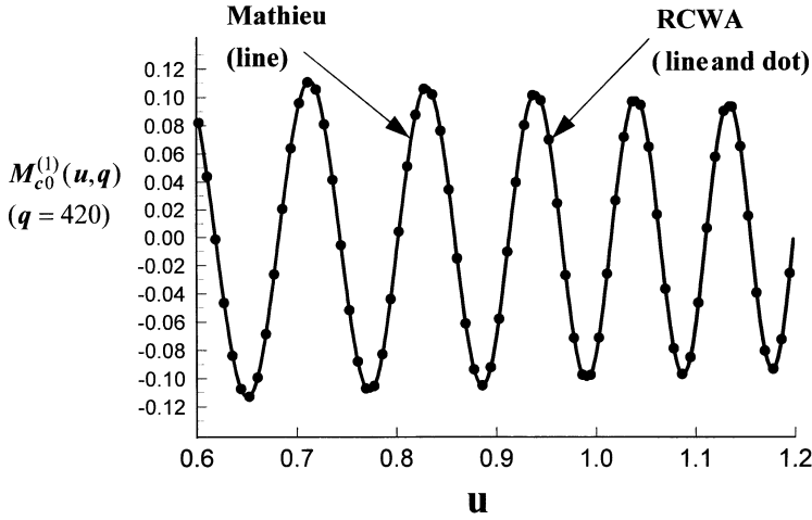
Figure 4. A comparison of the M_{c0}^{(1)}(u, q) radial Mathieu function as calculated by [21] and as calculated by RCWA is shown for q = 420 .
