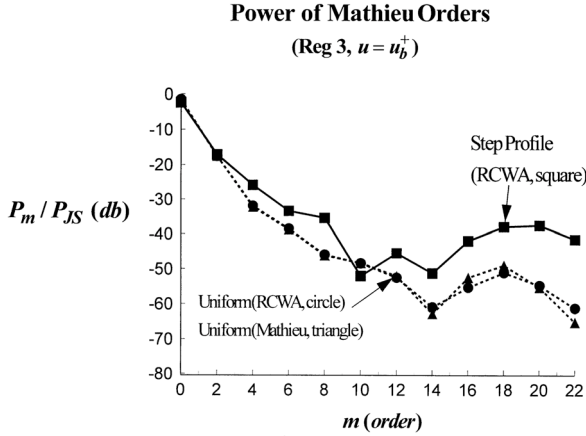
Figure 8. A display of the power ratio in db (using the db power formula 10 \log(P_m / P_{JS}) ) of the different Mathieu orders ( m = 0, 2, 4, \dots, 22 ) for the uniform elliptical shell case (using the Mathieu matching and RCWA methods) and the step profile case (RCWA) calculated in Reg. 3 at u = u_b^+ is shown. When Reg. 1 is infinite and \varepsilon_1 = 1. , \mu_1 = 1. , it turns out that the total power radiated from \vec{J}_S(u_s, v) of Eq. (35) is P_{JS} = 6.816674 \times 10^{-2} (Watts/m).
