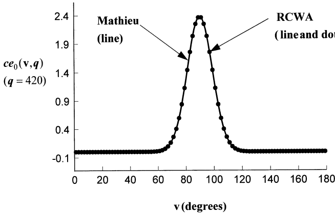
Figure 3. A comparison of the ce_0(v, q) angular Mathieu function ( line ) as obtained by the numerical algorithm of [21] and as obtained by the RCWA algorithm for q = 420 . This value of q (q = \mu\varepsilon\rho^2/4) would correspond to the case when \rho = 20 , \mu = 1.4 , \varepsilon = 3 .
