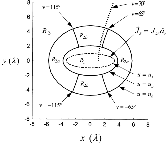
Figure 2. The geometry of the step profile, elliptical system is shown. The relative permittivity step profile is defined by; \varepsilon(x, y) = \varepsilon_{2a} = 2.95 in R_{2a} , (Reg. 2a) and \varepsilon(x, y) = \varepsilon_{2b} = 3.05 in R_{2a} (Reg. 2b). \varepsilon_{2U} has been chosen (see Fig. 1 caption) so \varepsilon_{2U} = (\varepsilon_{2a}S_{2a} + \varepsilon_{2b}S_{2b})/(S_{2a} + S_{2b}) where S_{2a} and S_{2b} are the areas of regions of R_{2a} and R_{2b} . All other parameters are specified in the Fig. 1 caption.
