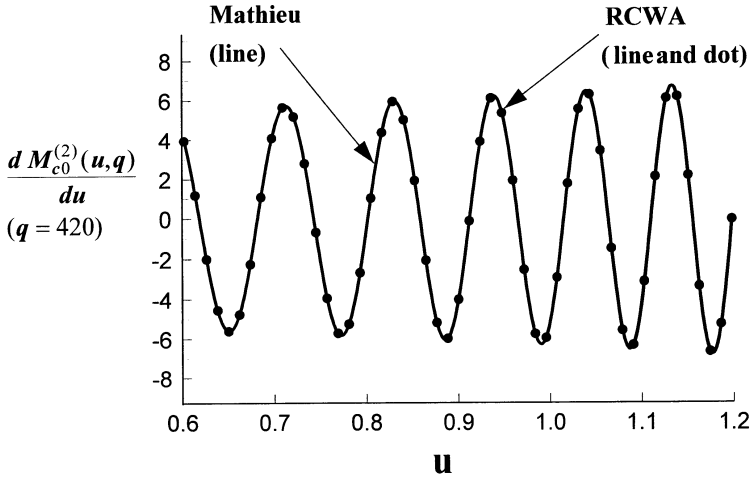
Figure 5. A comparison of the \frac{dM_{c0}^{(2)}(u, q)}{du} radial Mathieu function as calculated by [21] and as calculated by RCWA is shown for q = 420 .
