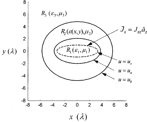
Figure 1. The geometry of the inhomogeneous elliptical system is shown where \rho = 20 , u_a = .602 , u_b = 1.198 , u_s = .3 , \lambda is the free space wavelength, and R_1, R_2, R_3 refer to Regs. 1, 2, 3 respectively. The figure is drawn to scale in the x and y directions. The relative permittivity \varepsilon(x, y) of Reg. 2 is assumed symmetric in the x and y coordinates. For all calculations is assumed: Reg. 1: \varepsilon_1 = 1. , \mu_1 = 1. ; Reg. 3: \varepsilon_3 = 1.5 , \mu_3 = 1.2 ; and for the uniform profile example it is assumed \varepsilon(x, y) = \varepsilon_2 \equiv \varepsilon_{2U} = 2.9851786 and \mu_2 = 1.4 .
