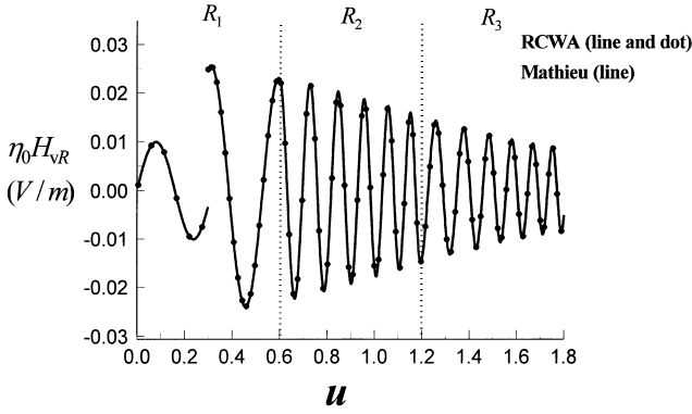
Figure 6. A comparison of \eta_0 H_{vR} ( \eta_0 = 377\Omega , H_{vR} is the real part of the phasor magnetic field the H_v ) for interval \rho = 20 , 0 < u \leq 1.8 with v = 70^\circ as obtained by a Mathieu expansion method of Sec. 3 and as obtained by RCWA algorithm of Sec. 2. Please see Fig. 2 for an x - y line plot of u for \rho = 20 , v = 70^\circ .
