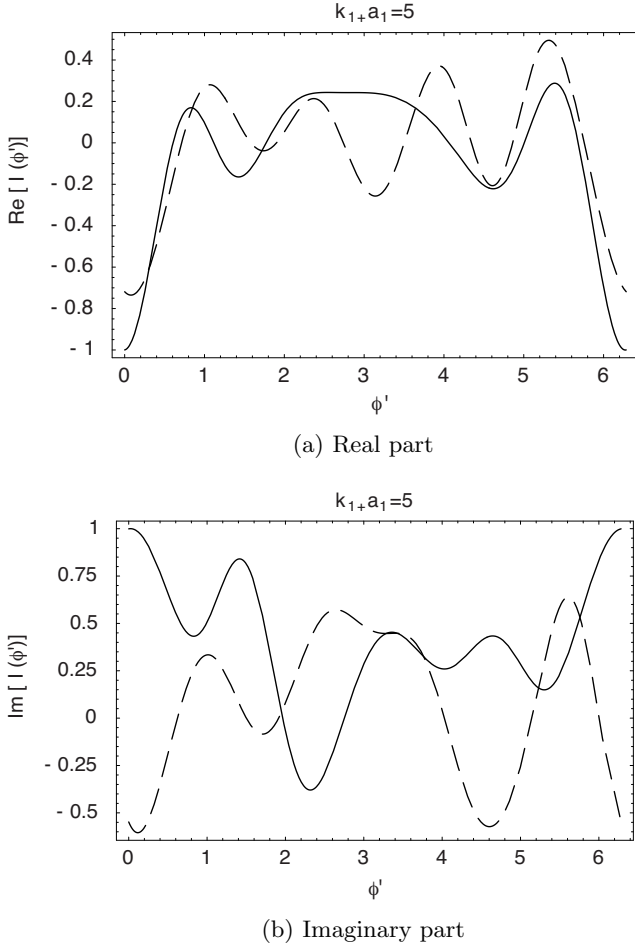
Figure 4. Current distributions for k_{1+}a_1 = k_{1-}a_1 = k_0a_1 = 5 . Solid and dash curves represent the results from utilizations of \mathbf{E}^{trans} and \mathbf{E}^{inc} , respectively.
