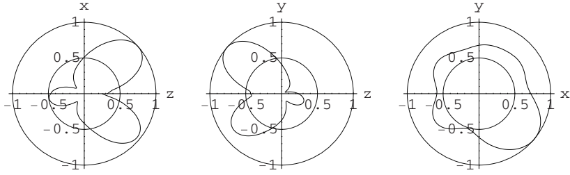
Figure 11. Field patterns for \xi = 5 \times 10^{-3} and k_0a_1 = 3 .
