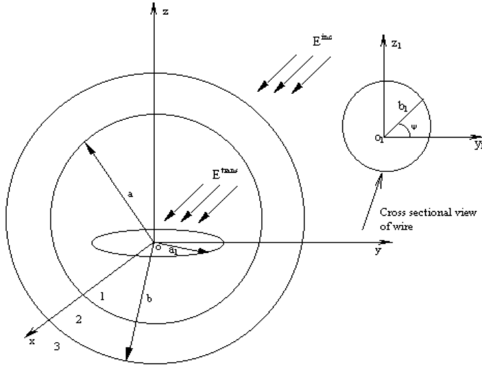
Figure 1. Geometry of a thin circular conducting loop in a two layered medium whose intermediate shell is a chiral radome.
