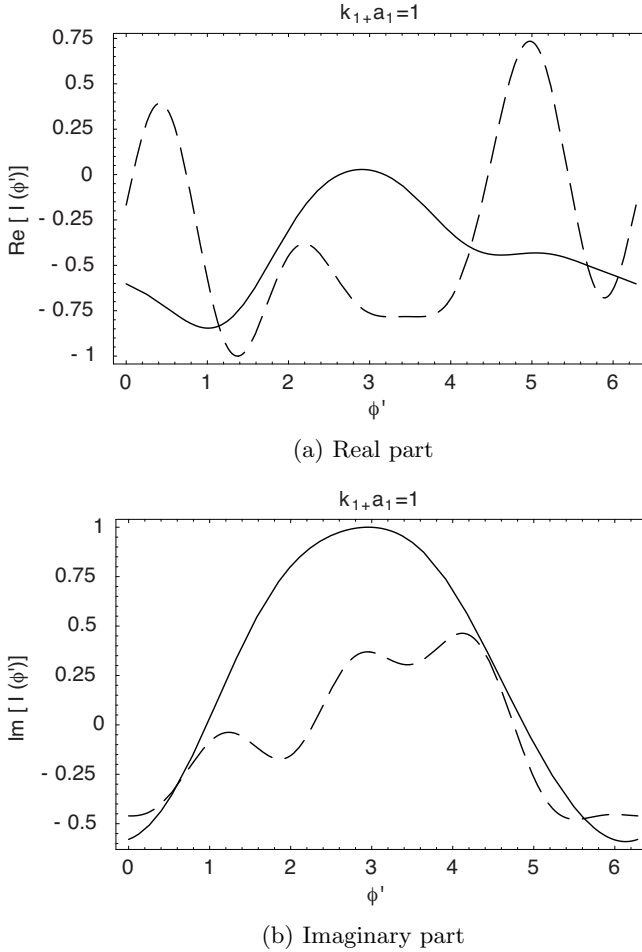
Figure 2. Current distributions for k_1+a_1 = k_1-a_1 = k_0a_1 = 1 . Solid and dash curves represent the results from utilizations of \mathbf{E}^{trans} and \mathbf{E}^{inc} , respectively.
