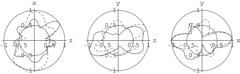
Figure 7. Field patterns for k_0 a_1 = 5 . Solid and dash curves represent the results from utilizations of \mathbf{E}^{trans} and \mathbf{E}^{inc} , respectively.
