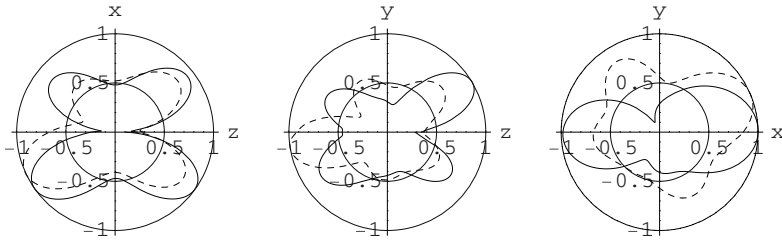
Figure 6. Field patterns for k_0 a_1 = 3 . Solid and dash curves represent the results from utilizations of \mathbf{E}^{trans} and \mathbf{E}^{inc} , respectively.
