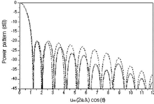
Figure 17. Symmetric sum pattern similar to a Rhodes pattern obtained with a smooth aperture distribution in Section 3.7 (—), and the original -20 dB \pi = 9 Rhodes pattern used as starting point.
