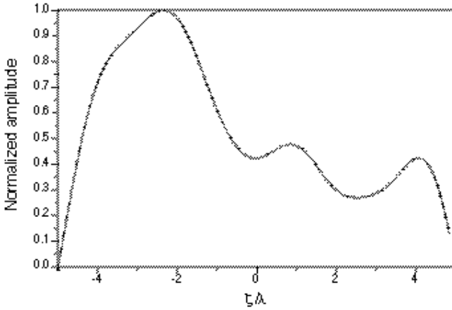
Figure 12. Amplitude of the aperture distribution affording the radiation pattern of Fig. 11.
