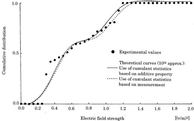
Figure 3. Evaluation of the cumulative distribution for the electric field based on cumulant statistics.
