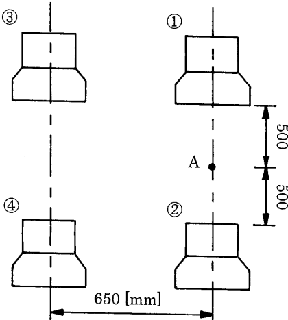
Figure 2. Arrangement of personal computers.
