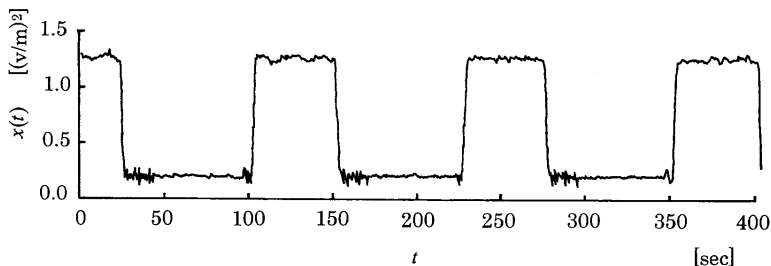
Figure 1. Fluctuation wave form of electric field.
