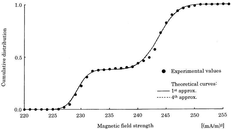
Figure 4. Estimation of the cumulative distribution for the magnetic field based on a stochastic exclusive property.
