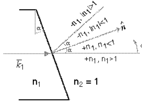
Figure 12. Possible directions of propagation for waves leaving a prism of material \epsilon_1 into free space.
