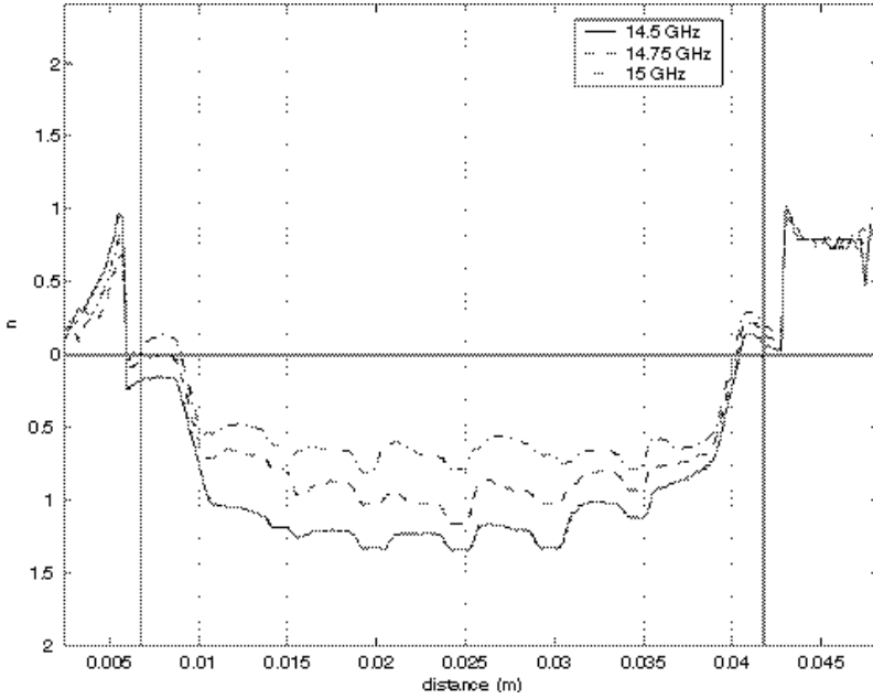
Figure 10. Index of refraction through Type 1 metamaterial for different frequencies.
