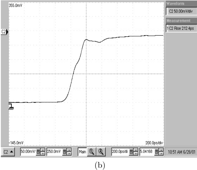
Figure 12. (a) Prediction of the driving signal distortion, and (b) measured driving signal waveform at the output of the active line.
