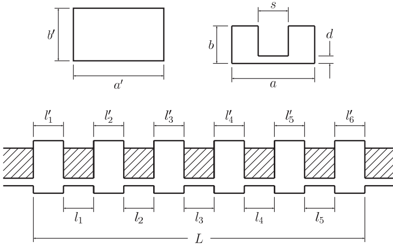
Figure 6. Dimension notations used in Tables 1 and 2 for the five-section 1-GHz filter.
