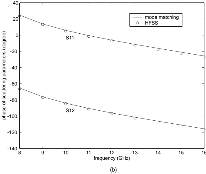
Figure 3. Scattering parameters of a structure composed of two identical back-to-back cascaded empty-to-ridge waveguide discontinuities. (a) Magnitude. (b) Phase. The structure dimensions in mils are: a = 180 , b = 80 , s = 36 , d = 12 , a' = 210 , b' = 80 , a_0 = 30 , b_0 = 0 , and l' = 100 . The structure is dielectric-filled ( \epsilon_r = 6 ).
