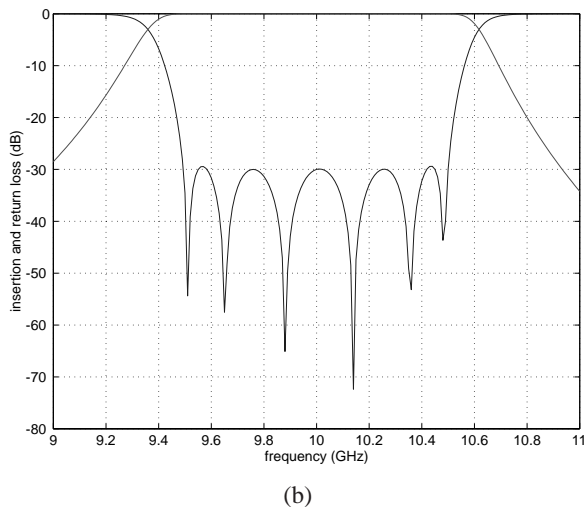
Figure 12. (a) Dimensions (given in mils) of half the six-section 10-GHz filter. Only half dimensions are shown here since the filter is symmetric with the folded junction. The structure is dielectric-filled ( \epsilon = 5.76 ). (b) Computed response of the six-section 10-GHz filter.
