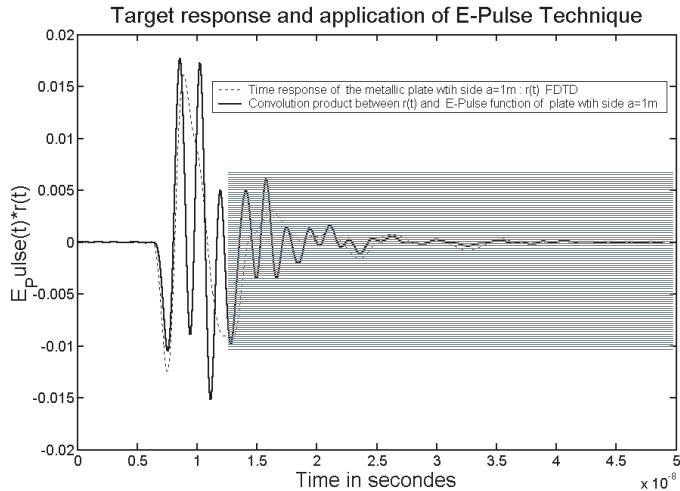
Figure 3b. Response of a metallic plate and and application of E -Pulse method.
