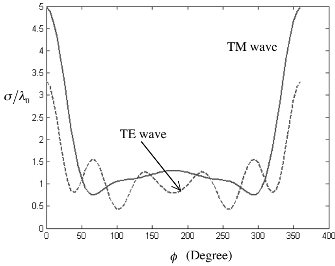
Figure 9. Normalized bistatic echo width of a metamaterial dielectric coated cylinder. ( a = 50 mm, b = 100 mm, \varepsilon_{r1} = -9.8 , \mu_{r1} = -1 , \phi_0 = 0^\circ and f = 1 GHz).
