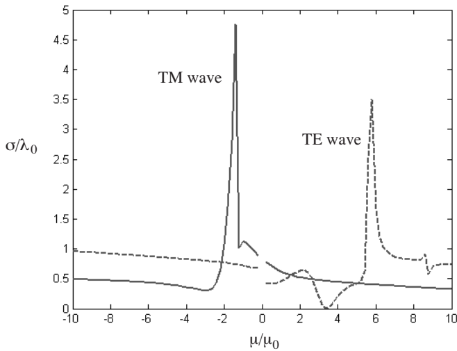
Figure 7. The back scattered cross section of a dielectric coated cylinder. ( a = 50 mm, b = 70 mm, f = 1 GHz, \varepsilon/\varepsilon_0 = -2.2 when \mu/\mu_0 < 0 and \varepsilon/\varepsilon_0 = 2.2 when \mu/\mu_0 > 0 ).
