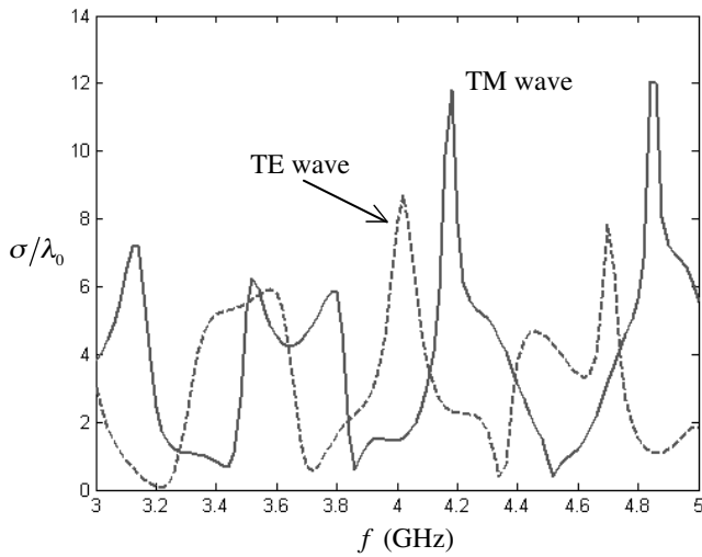
Figure 10. The backscattered cross section of a normal dielectric coated cylinder. ( a = 50 mm, b = 100 mm, \varepsilon_{r1} = 2.54 and \mu_{r1} = 1 ).
